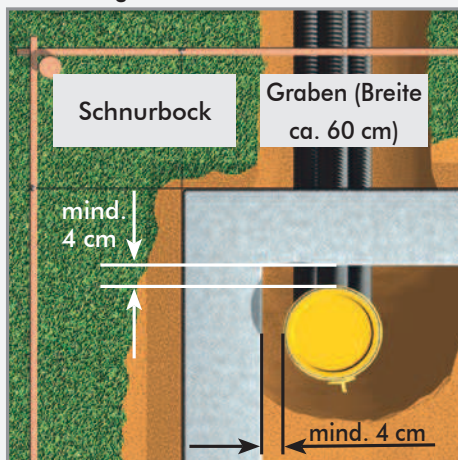
Abb. 8: Quadro-Secura® Nova BP-R
